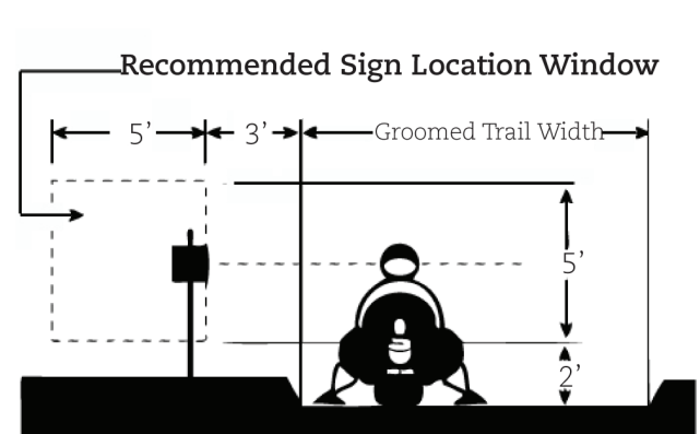
Figure 3 - Recommended sign location window
